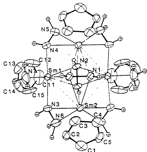
Figure 1. Molecular structure of [\text{Cp}^*\text{Sm}]_4(\text{NHNH})_2-(\text{NHNH}_2)_4(\text{NH}_3)_2 viewed parallel to the 2-fold axis, with probability ellipsoids drawn at the 50% level. \text{Cp}^* methyl groups have been omitted for clarity. (Reprinted from ref 263. Copyright 1992 American Chemical Society.)
